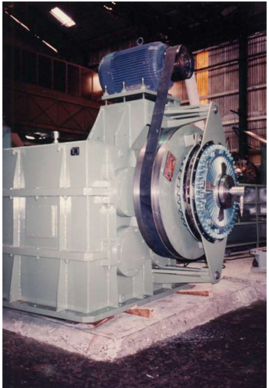
Speed reducer with pneumatic clutch and two output shafts for shovels manufacturing
